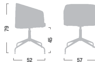
MN13 Poltroncina girevole, base a 4 razze. Four beam revolving chair.
