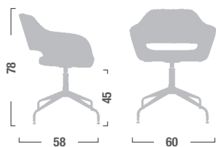
FL12 Poltroncina girevole, base a 4 razze. Four beam revolving chair.
