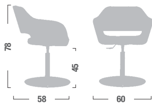
FL10 Poltroncina girevole, base a calice. Globed base revolving chair.
