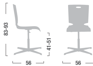
BR26 Sedia girevole, base a 4 razze. Four beam revolving chair.
