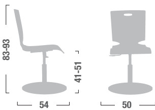
BR29 Sedia girevole, base a calice. Globet base revolving chair.
