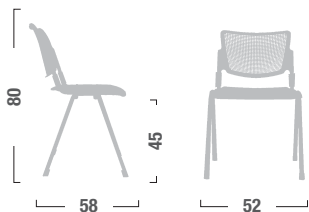
LA10 Sedia fissa a 4 gambe. Four legs fixed chair.
