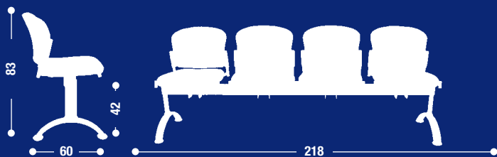
Panca a 4 posti Four seater bench
